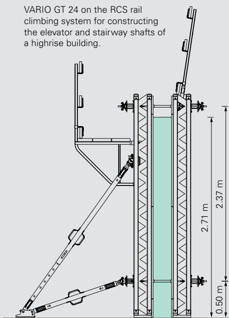
VARIO panels, with concreting scaffold and push-pull props, are shifted as a complete unit.
